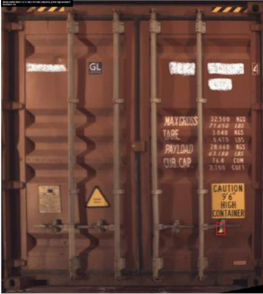
Figure 3. Sealed Container
