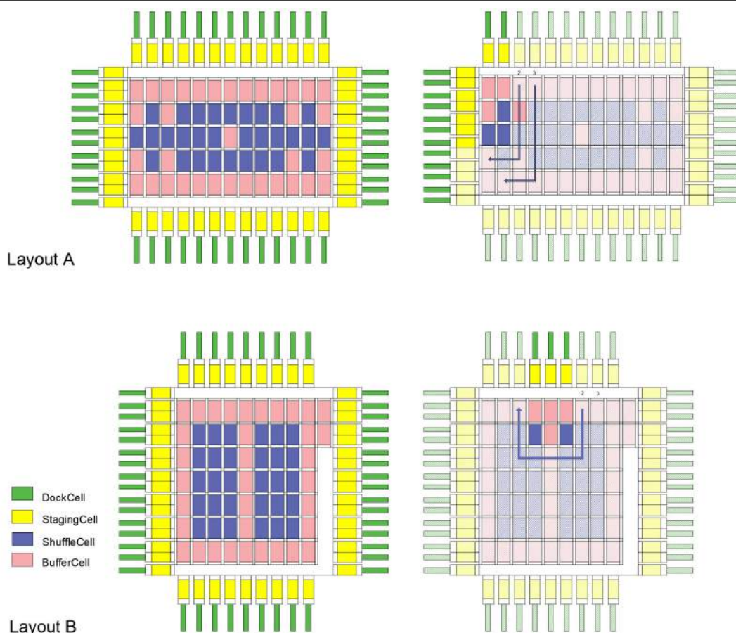
Figure 15: HLH Layouts Depicted with Dynamic Variations of Activated and Disactivated Cells
