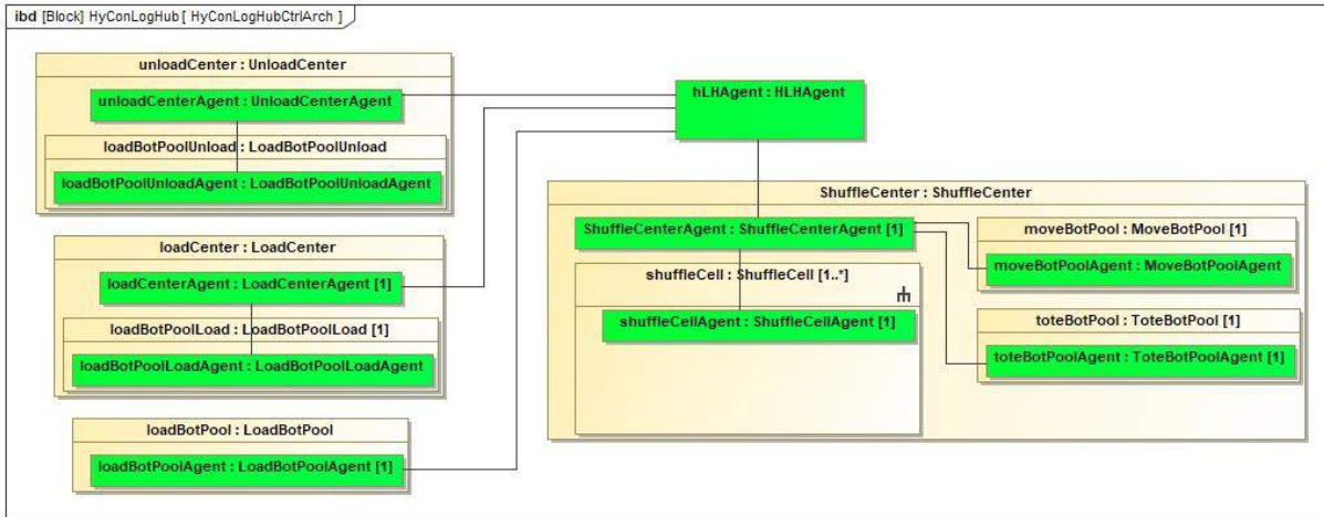
Figure 2 HLH Control Architecture
