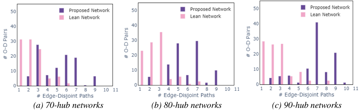
Figure 3: Edge-disjoint path distribution for the proposed and lean networks
