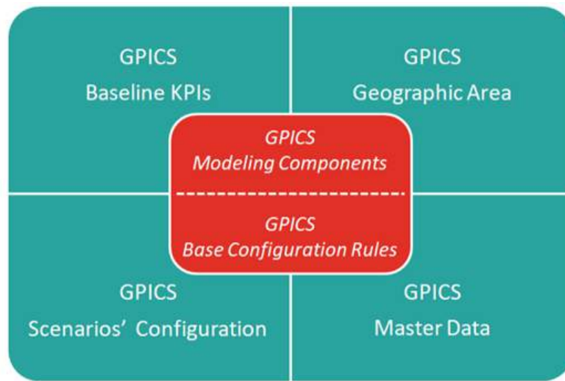
Figure 1: GPICS Framework/Dimensions
